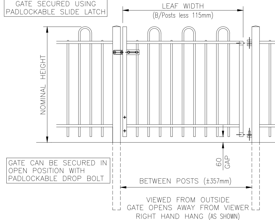
PEDESTRIAN SINGLE GATE WITH SLIDE LATCH
