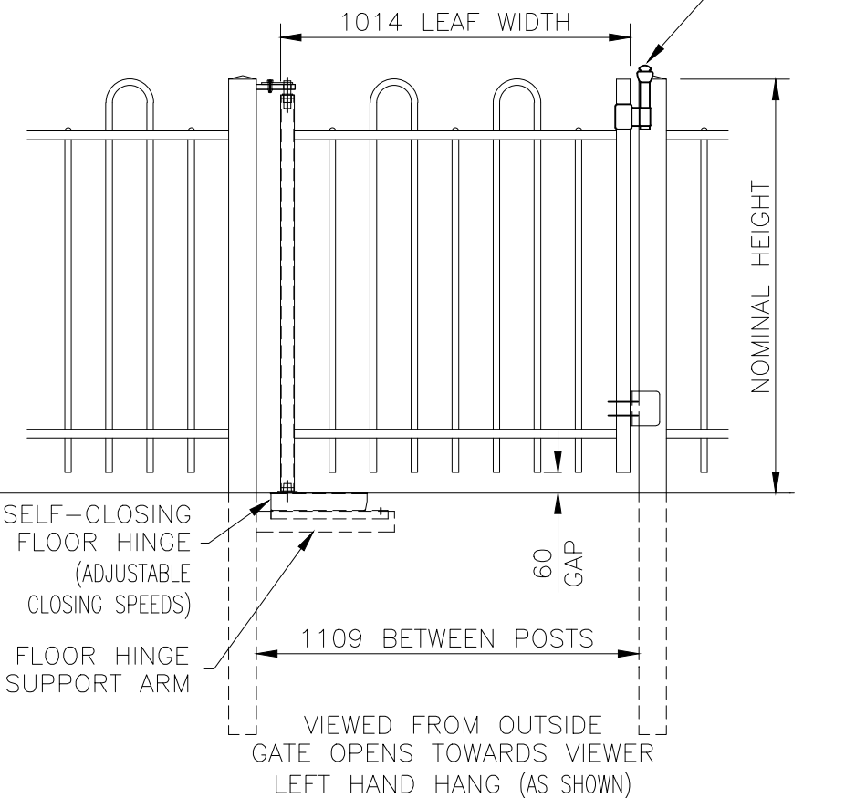
SELF CLOSING SINGLE GATE
